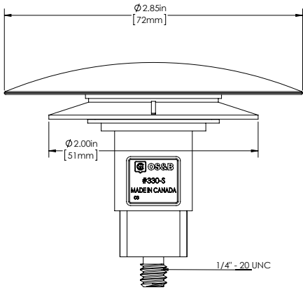
332/332B( )-S. Featuring a 1/4\"-20 UNC thread post. Fits Waste/Overflow fine thread strainers.
