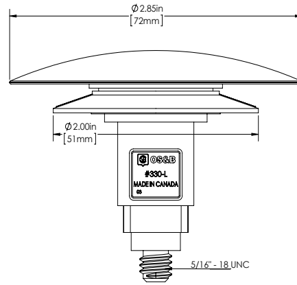
332/332B( )-L. Featuring a 5/16\"-18 UNC thread post. Fits Waste/Overflow coarse thread strainers.
