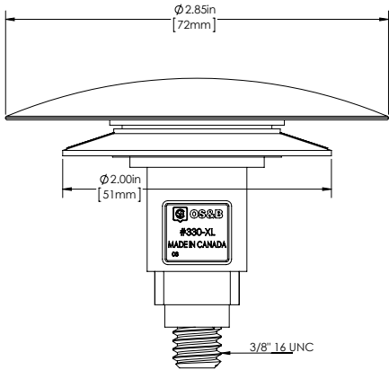
332/332B( )-XL. Featuring a 3/8\"-16 UNC thread post. Fits Waste/Overflow extra-coarse thread strainers.
